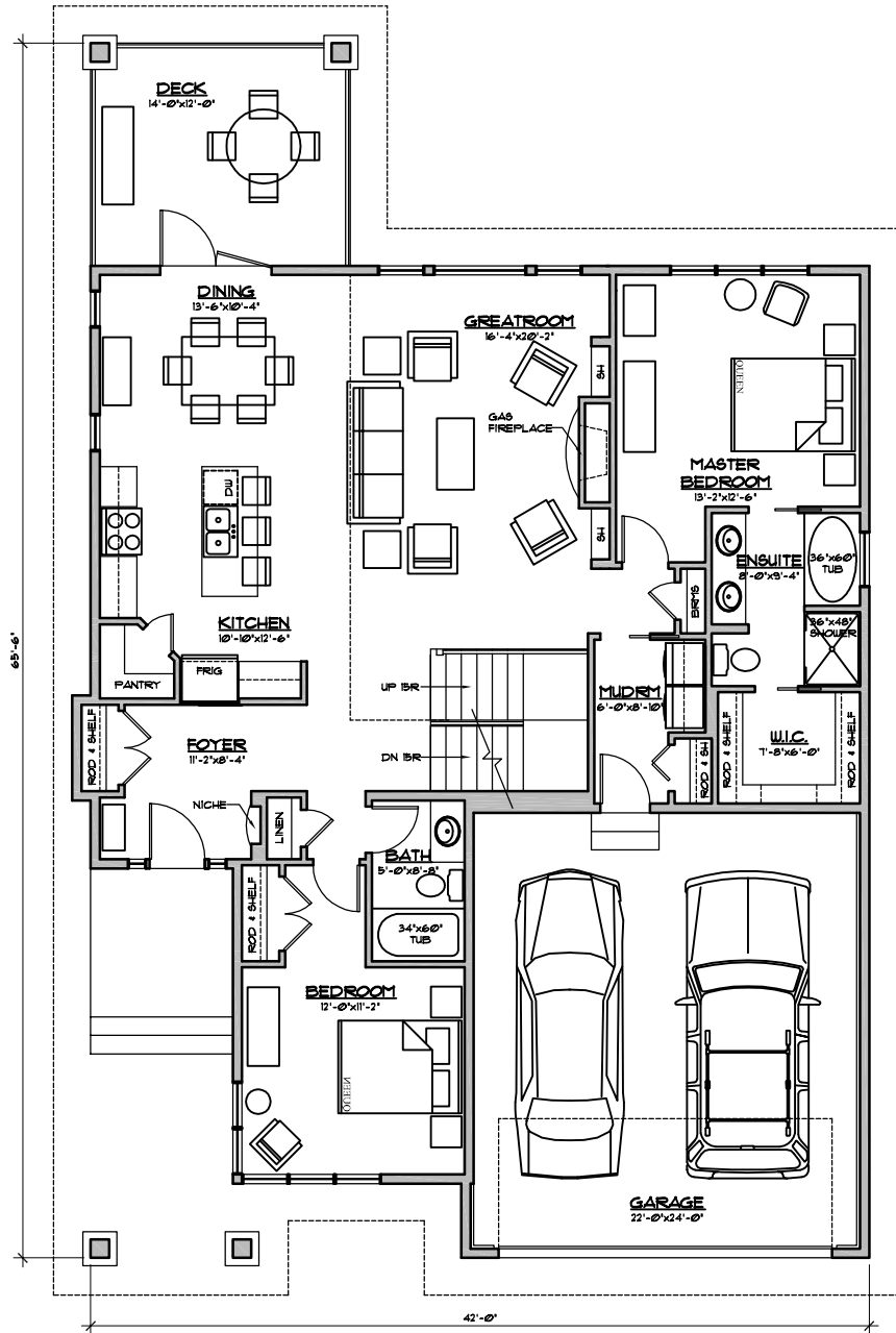
MAIN FLOOR PLAN SCALE: NTS AREA: 1528 SQ FT
