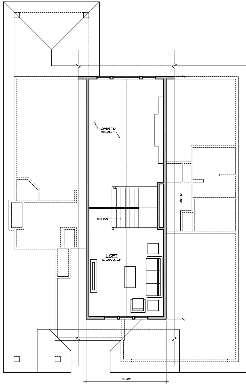
LOFT PLAN SCALE: NTS AREA: 354 SQ FT
