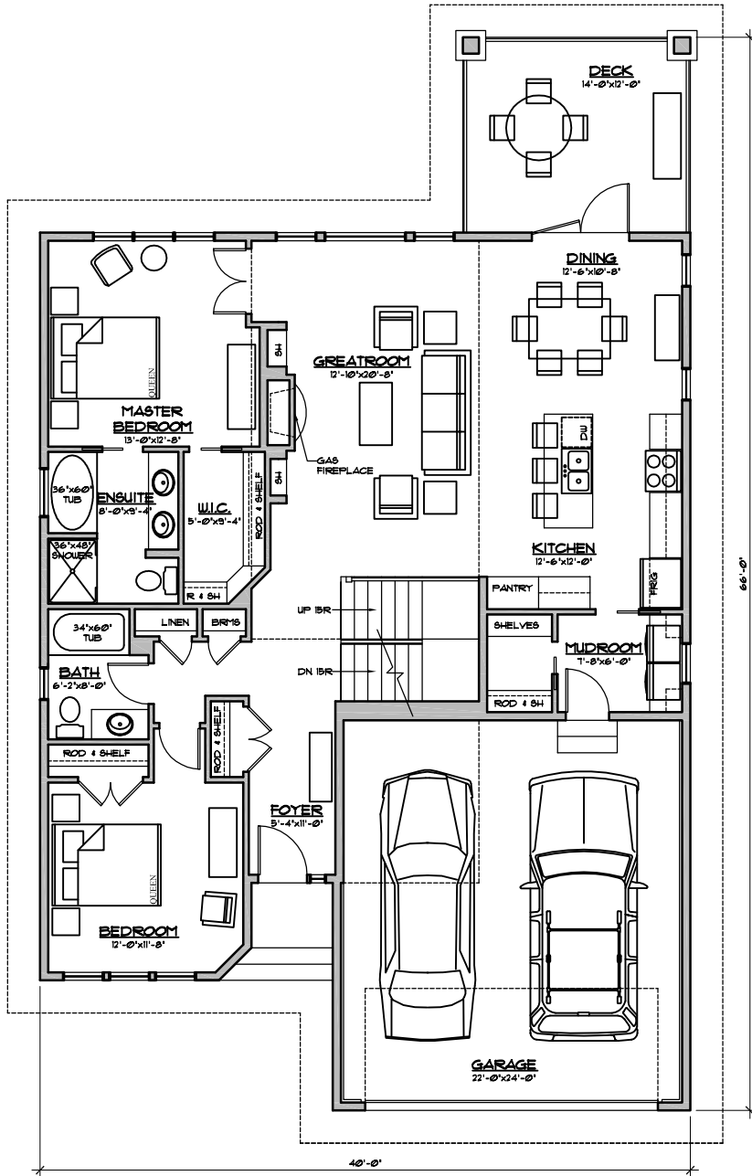
MAIN FLOOR PLAN SCALE: NTS AREA: 1463 SQ FT
