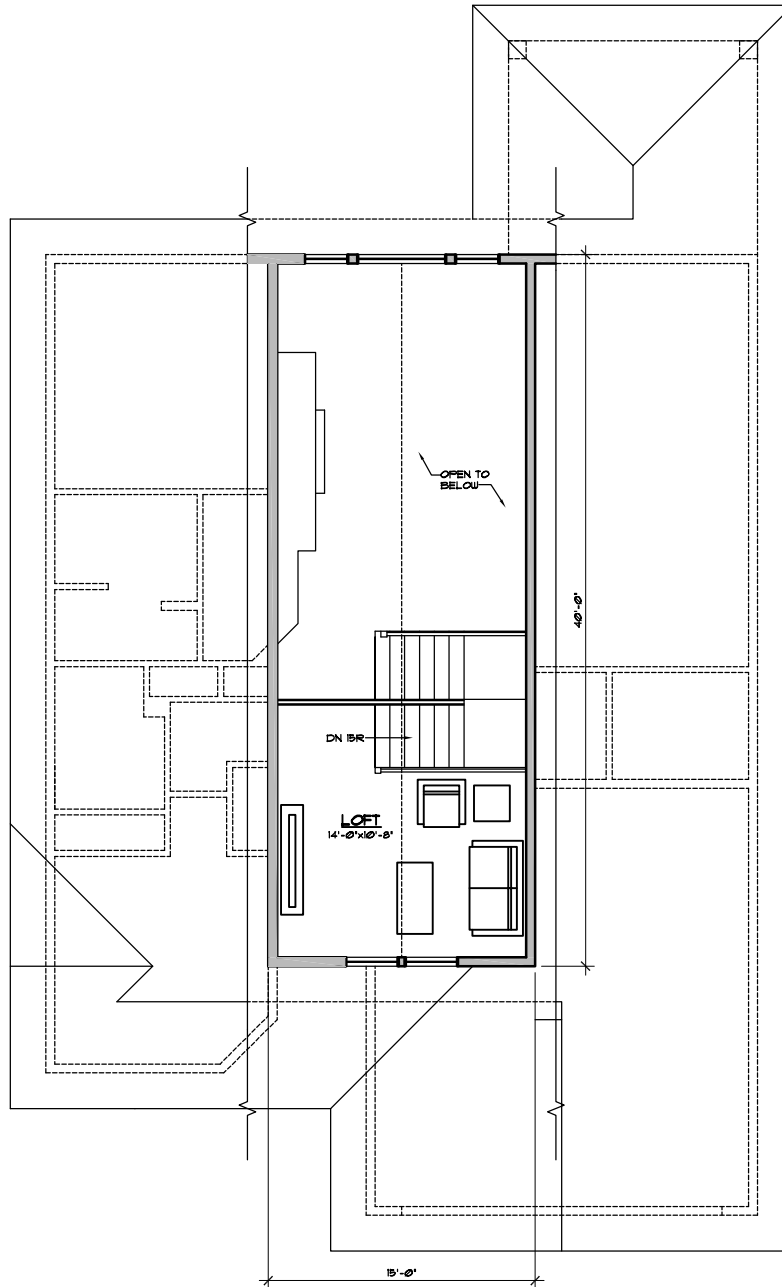
LOFT PLAN SCALE: NTS AREA: 225 SQ FT
